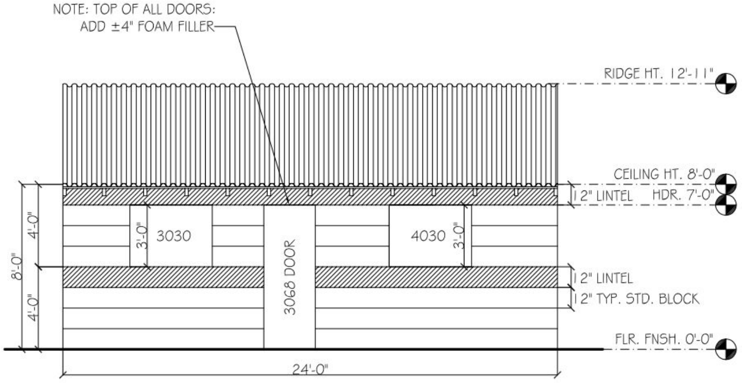
ELEV. 1 (FOAM BLOCK LAYOUT - LINTELS/HEADERS AT 4' AND 8')
